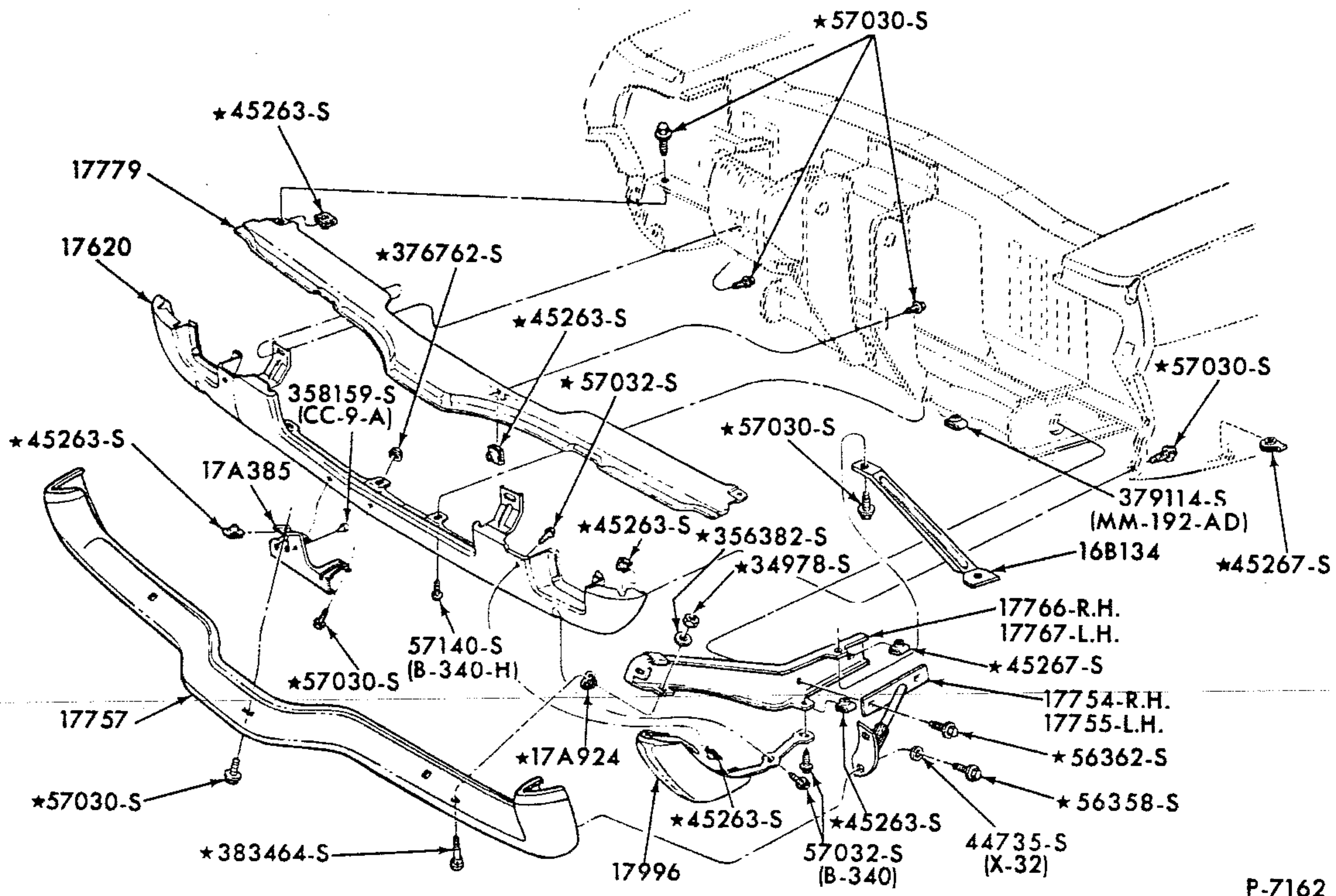
FRONT BUMPER and RELATED PARTS 1970 COUGAR
