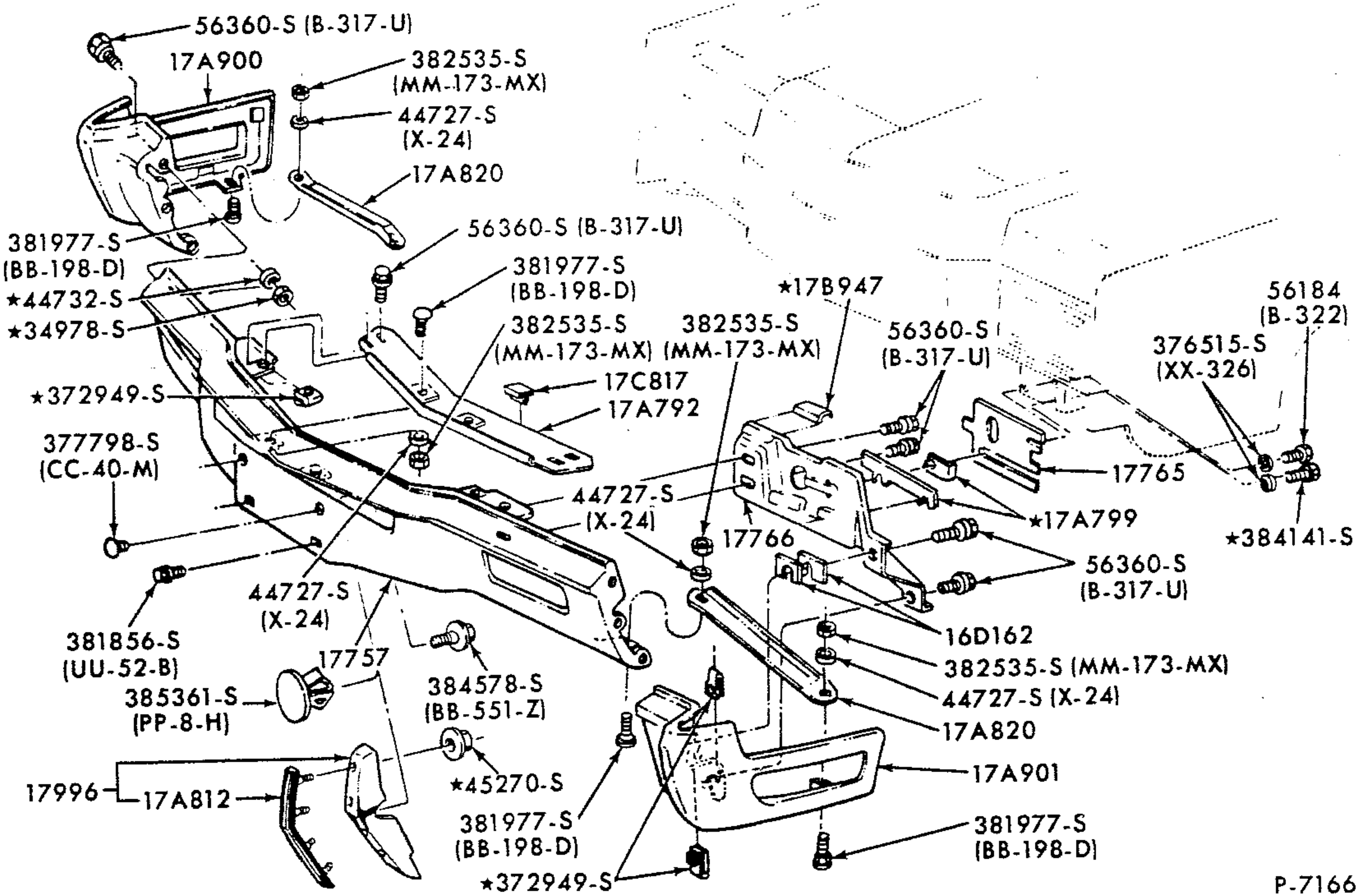
FRONT BUMPER and RELATED PARTS 1970/72 LINCOLN
