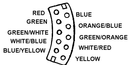
1968 Cougar Turn Signal Switch connector
