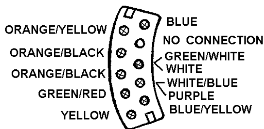
1968 Cougar Main harness Turn Signal Switch connector
