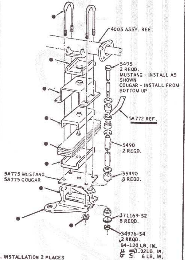
TYPICAL INSTALLATION 2 PLACES
